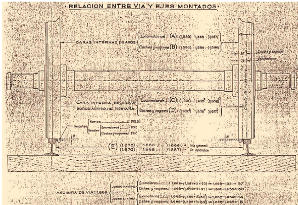
Relationship between track gauge and distance between wheels. (Source: "Track Play Reduction", Renfe's Department of Studies and Reconstruction, March 1995)
