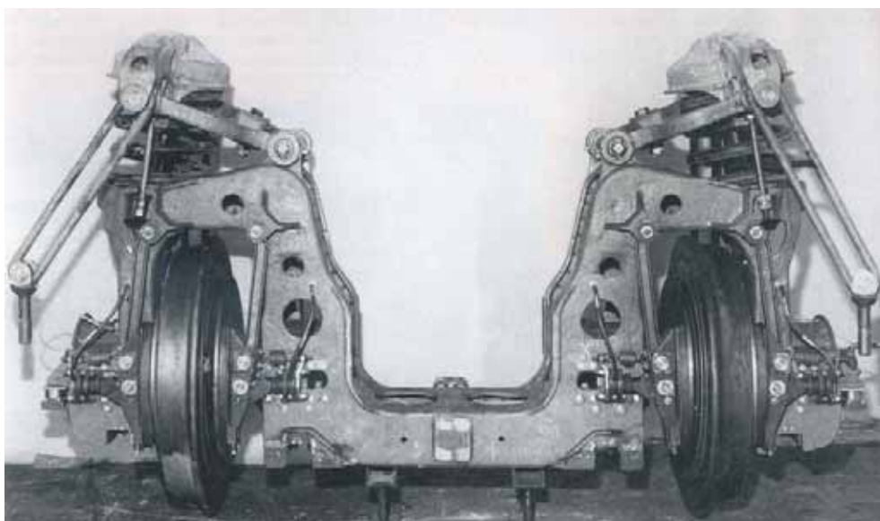
Talgo III RD variable gauge wheelset (1968). (Photo: Talgo)
